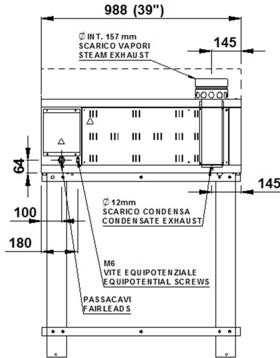
REAR VIEW
